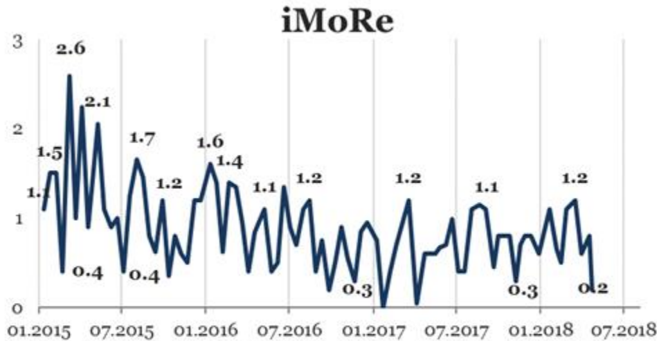
Chart 1. iMoRe dynamics*
